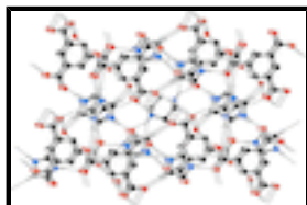
Fig. 2. Part of the title crystal structure, showing the three-dimensional network linked by N—H···O, O—H···O and C—H···O hydrogen bonds represented by dashed lines. For the sake of clarity, the H atoms not involved in the hydrogen-bonds pattern have been omitted. Color code: C, black; H, white; N, blue; O, red.
